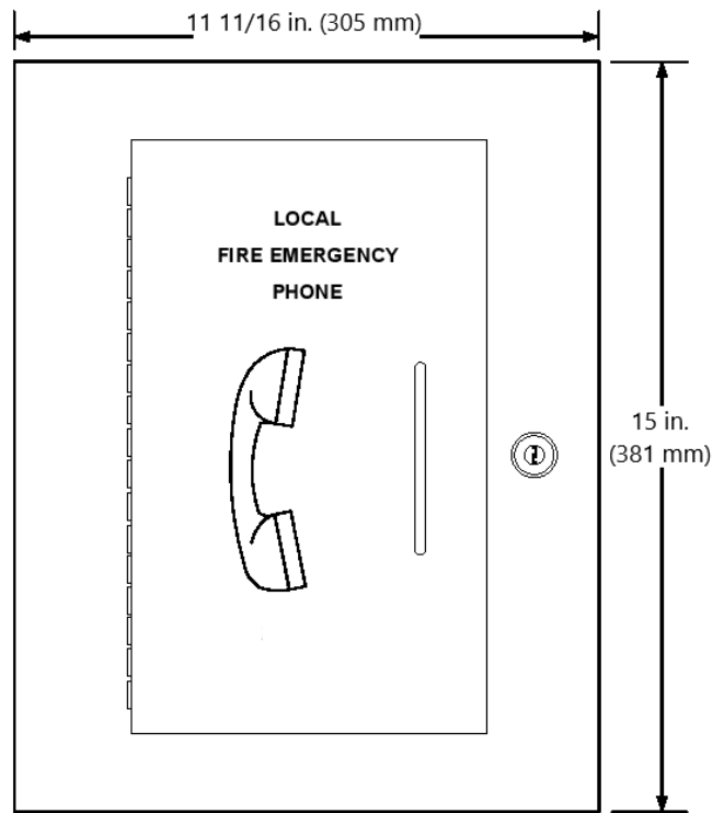
Figure 9: Flush Mount Assembly Reference
