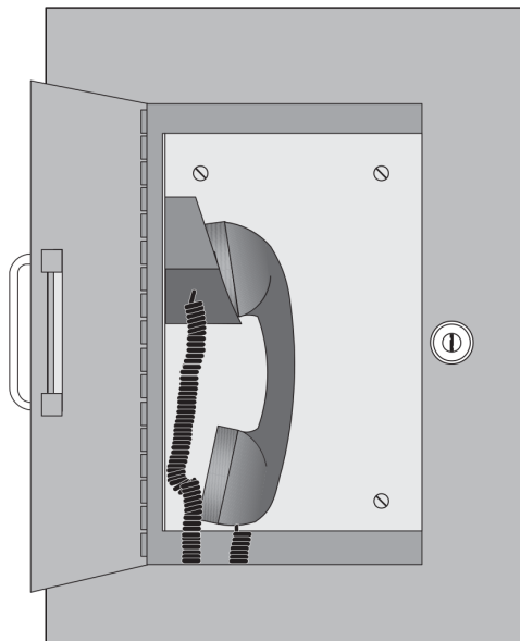
Figure 6: Interior View of Remote Phone Cabinet (Shown With Pull Handle and Break-rod)
