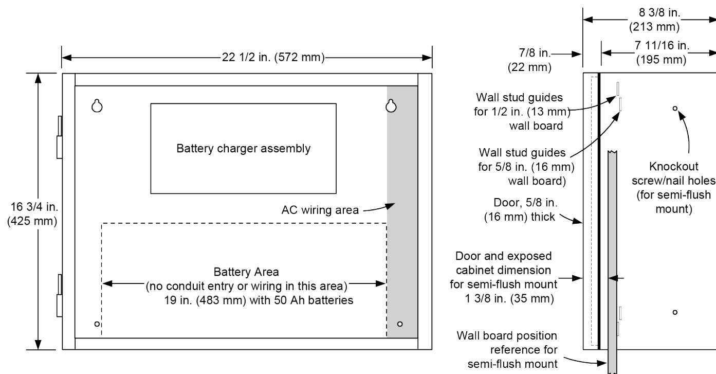
Figure 2: Installation reference
