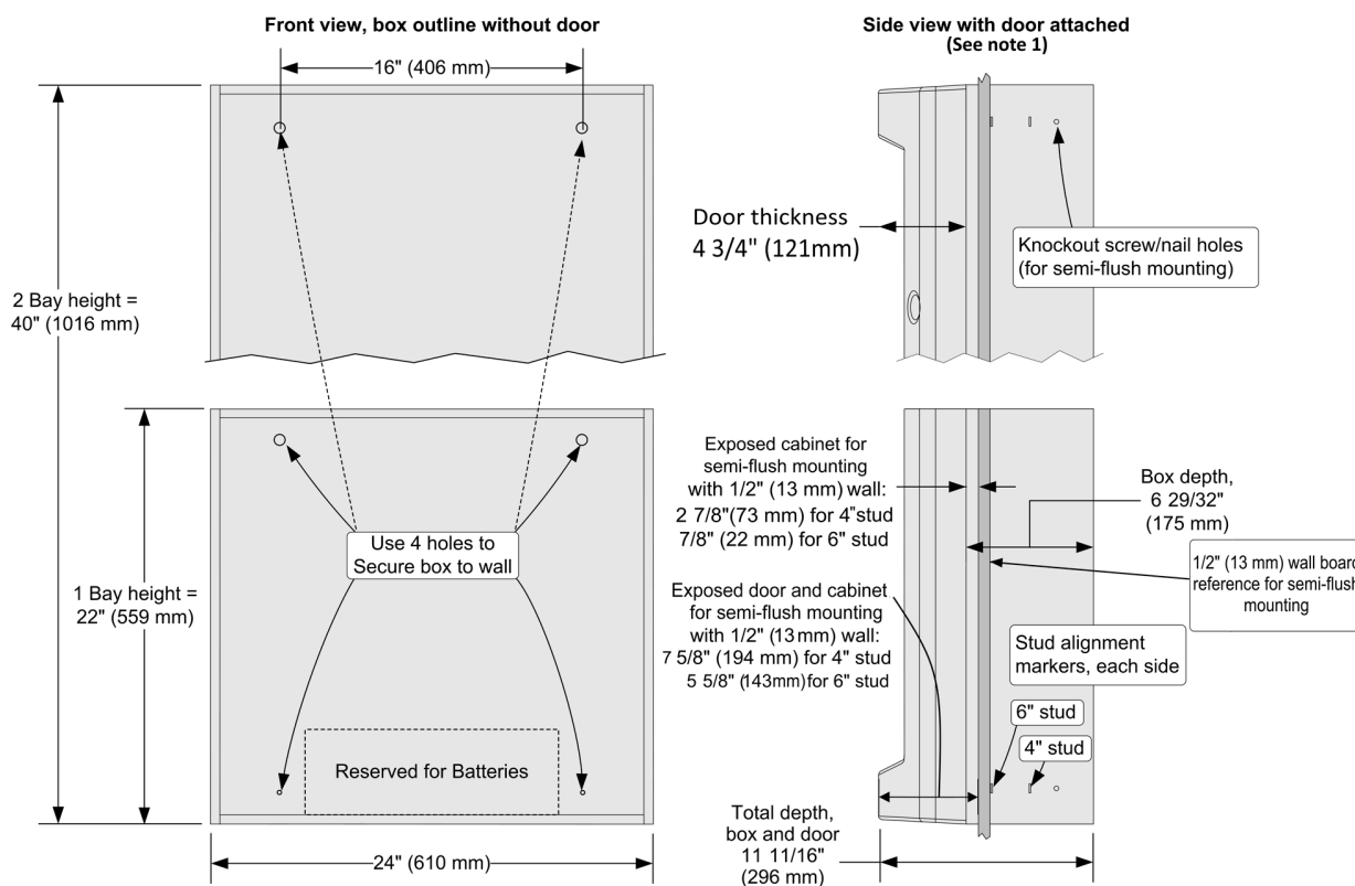
Figure 17: Cabinet dimensions
